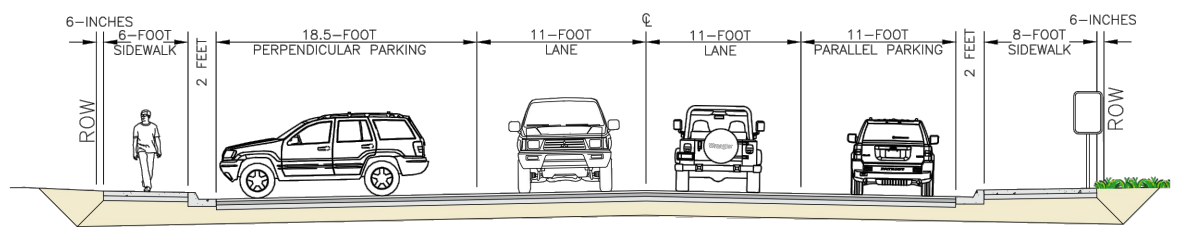
TYPICAL SECTION, BLOCK 3
